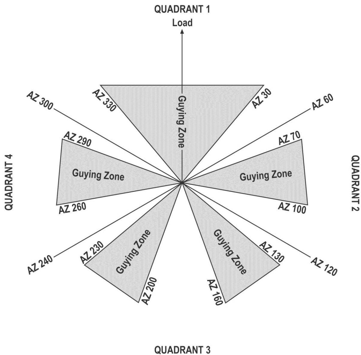
Figure 7-44 – 5 Guyline Case
