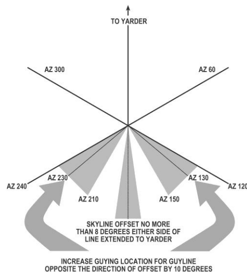
Figure 7-16 – Guylines – Tail Trees
