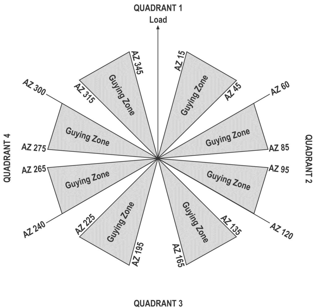
Figure 7-49 – 8 Guyline Case
