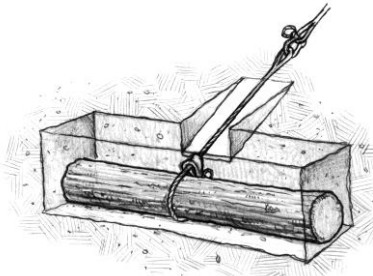
Figure 7-23 – Deadman Anchor
