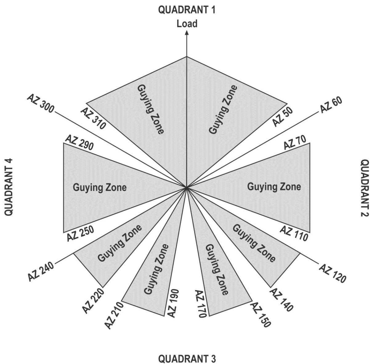
Figure 7-50 – 8 Guyline Case
