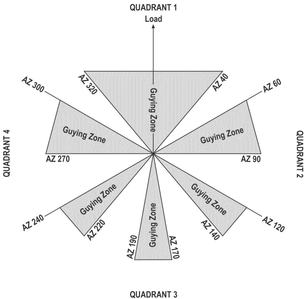
Figure 7-47 – 6 Guyline Case
