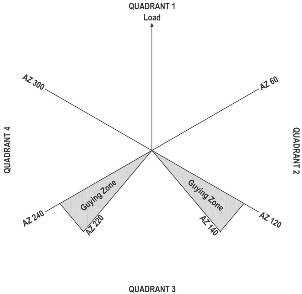
Figure 7-40 – 2 Guyline Case
